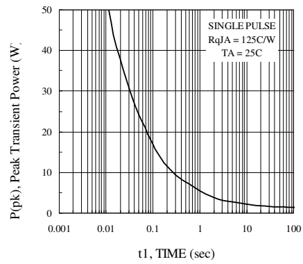
Figure 10. Single Pulse Maximum Power Dissipation
